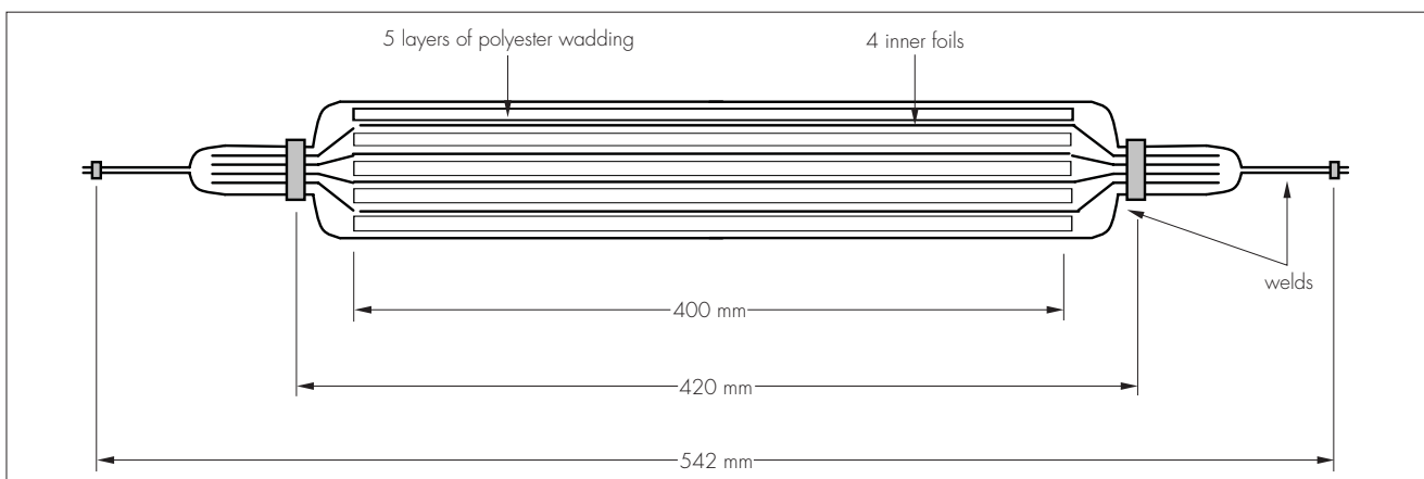
Figure 1 Rafterfit cross-section
